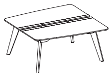
FS26 - 1600x1600x750h
